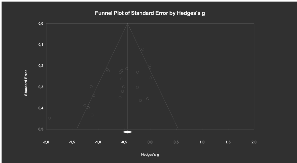
Figure 1. Funnel plot random effects ( k = 23 ).
